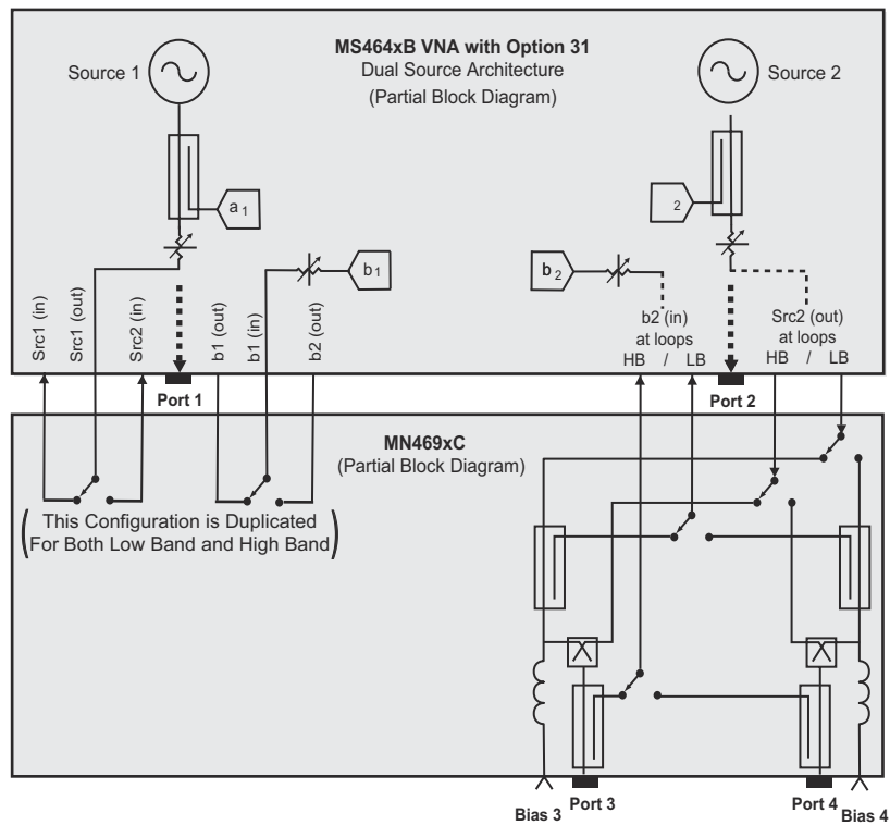
Figure 1-2. MS464xB VNA With Option 31 Dual Source Architecture
